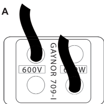
For this style power supply use wire configuration A.
