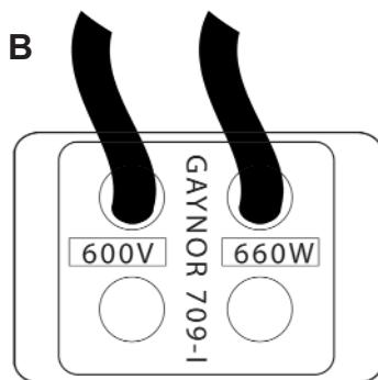
For this style power supply use wire configuration B.
